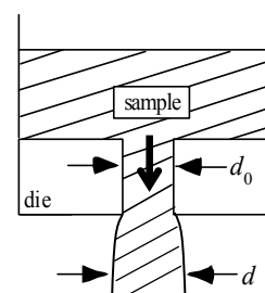
Fig.1 Schematic diagram of our extruding system.
