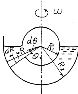
Fig.4 Analysis of fluid force on floating sphere
