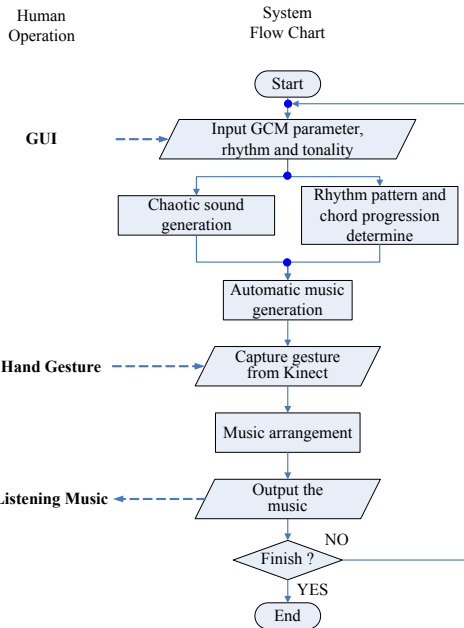
Fig. 2. Algorithm Of Proposed Music Generation System
