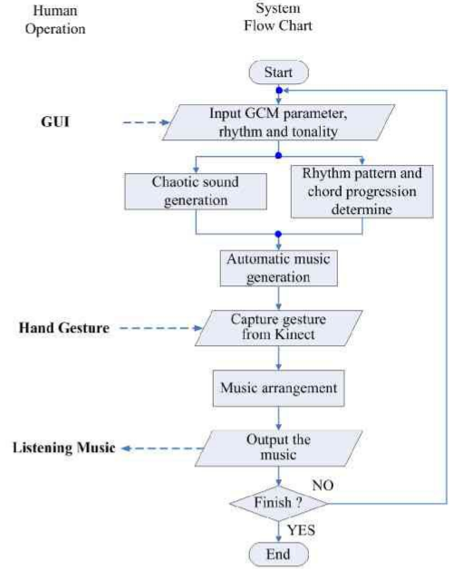
Fig. 2. Algorithm Of Proposed Music Generation System
