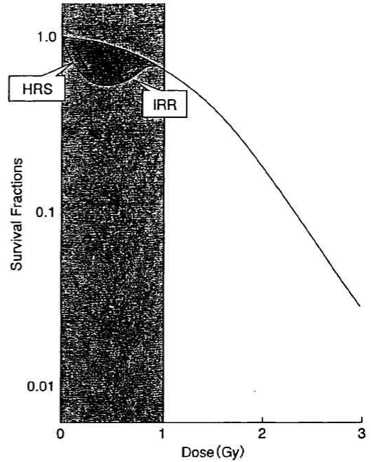
図1 Hyper-Radiosensitivity (HRS) と Increased Radioresistance (IRR)
